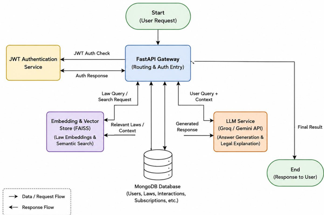
Figure 3.3 — System technical architecture
