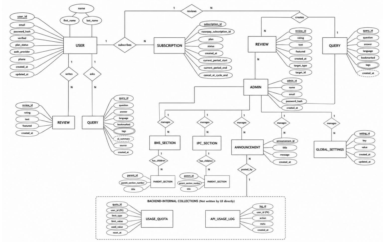
Figure 4.1 — Entity–Relationship Diagram — VidhanAI (Complete)
