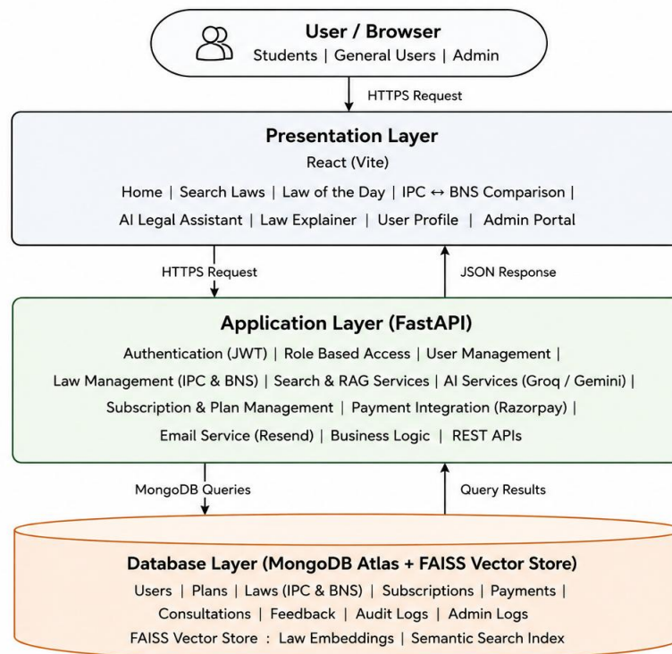
Figure 3.2 — System software architecture
