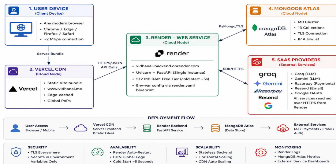
Figure 3.4 — System hardware architecture (deployment view)
